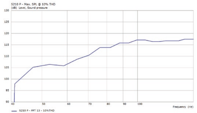
Max. SPL (blau = 10 % THD)
