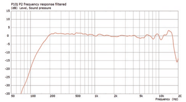
Frequenzgang (processed)
