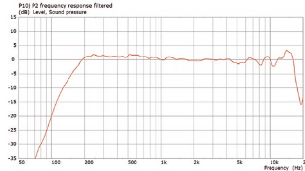
Frequenzgang (processed)
