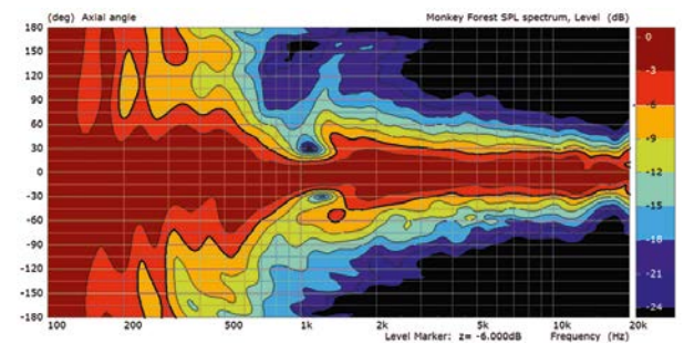
Vertical directivity
