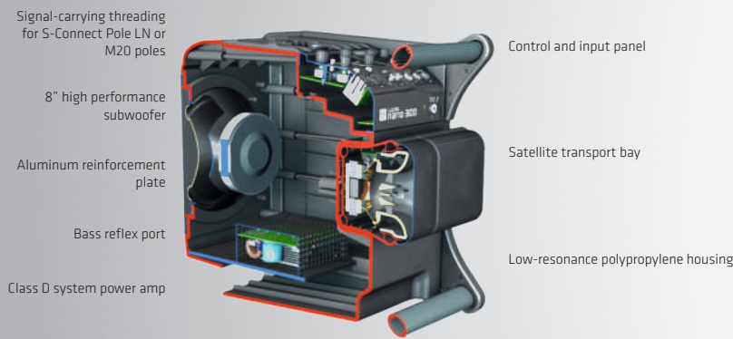
Cross-section of a LUCAS NANO 300 series subwoofer
