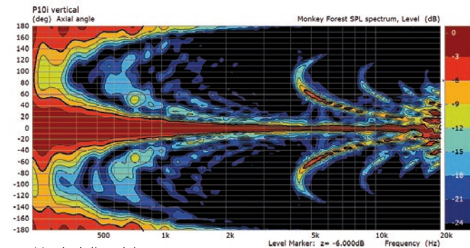
Vertical directivity
