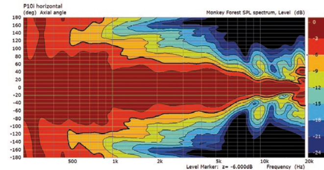
Horizontal directivity
