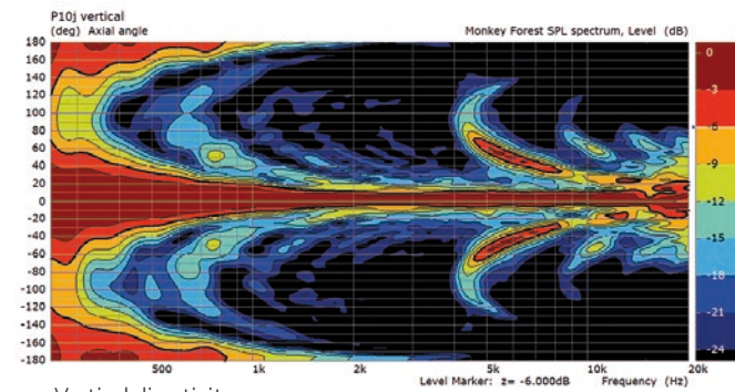
Vertical directivity
